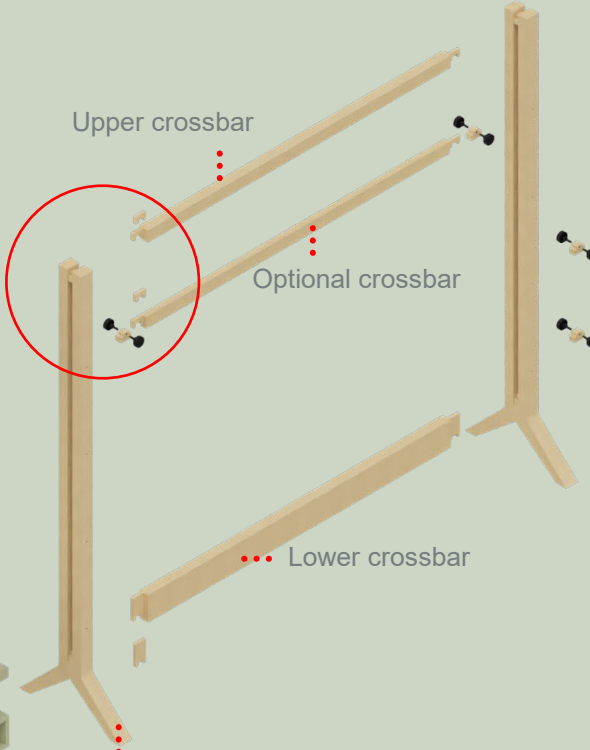
Side frame incl. 2 x T-connector
